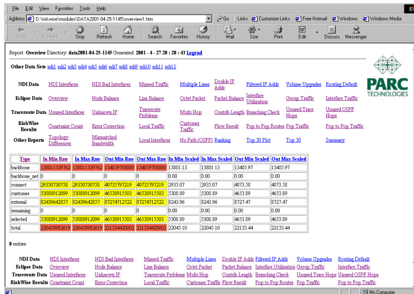
Figure 6.1: HTML Report
