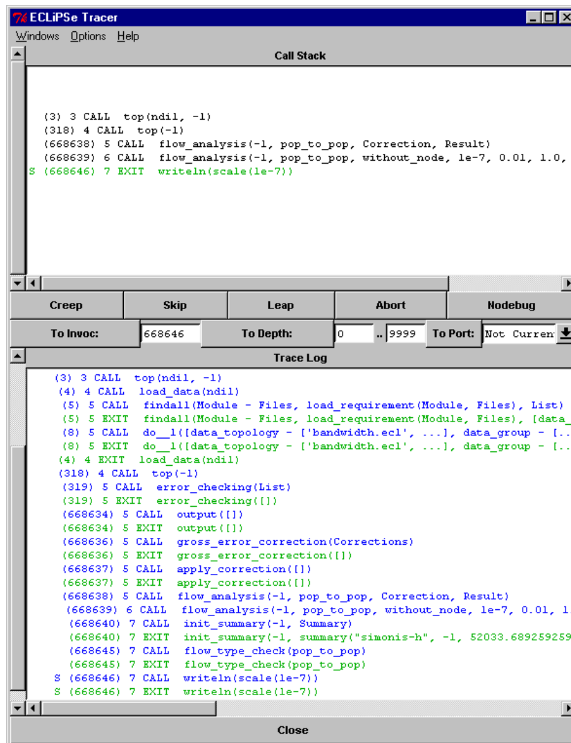
Figure 7.1: ECLiPSe Tracer
